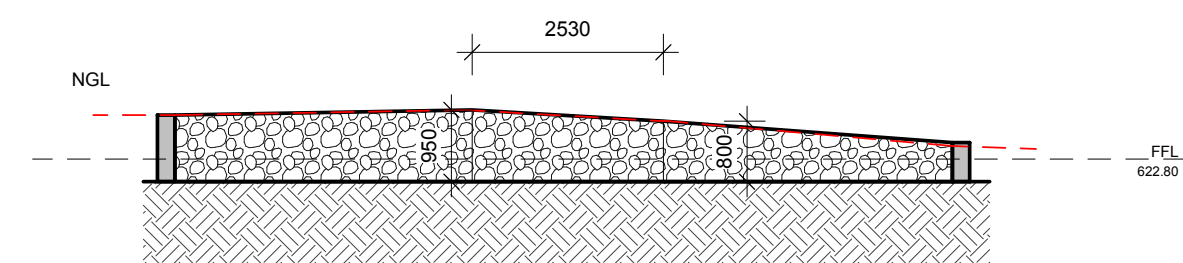
RETAINING F-F 1 : 100
