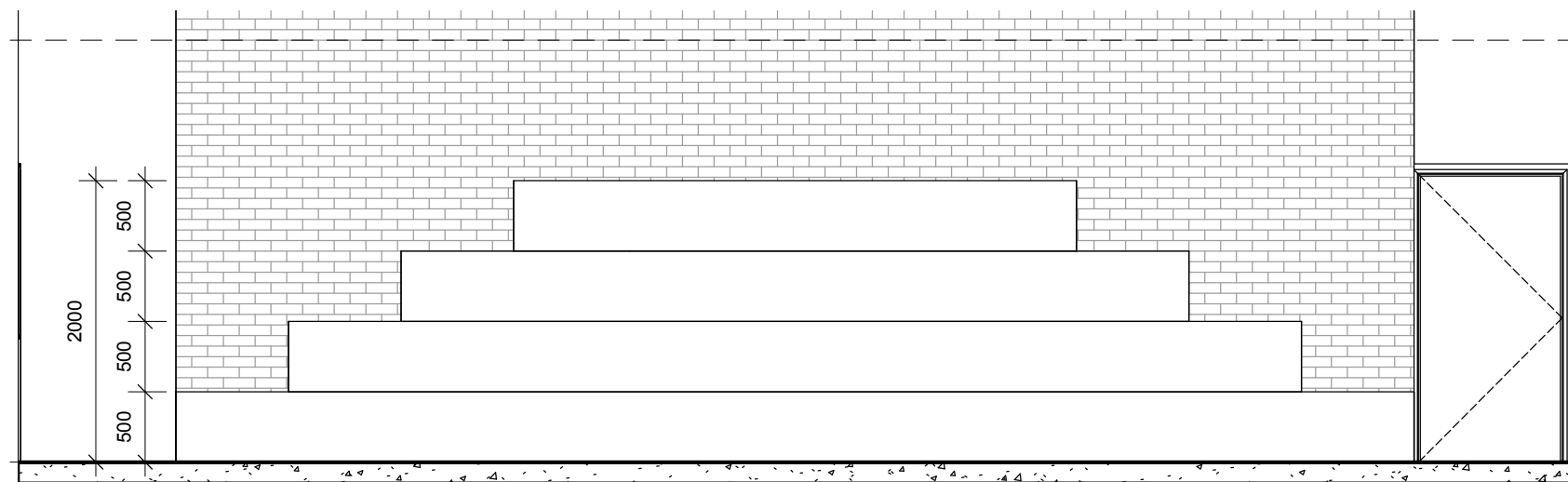
Altar Elevation 1 : 50
