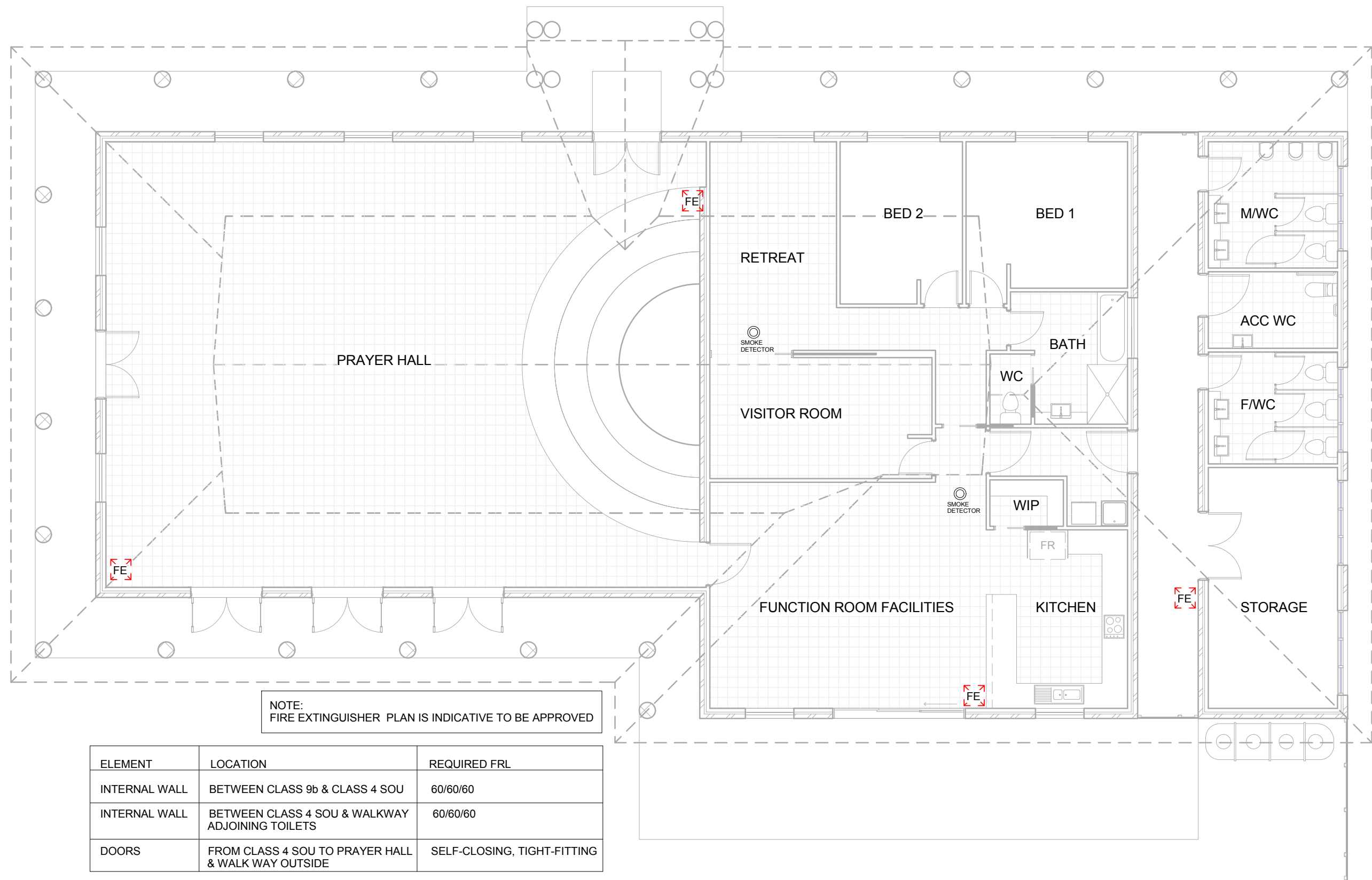
INDICATIVE FIRE PREPARATION PLAN 1 : 100
