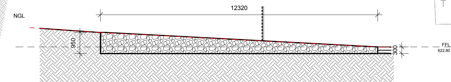
RETAINING E-E 1 : 100
