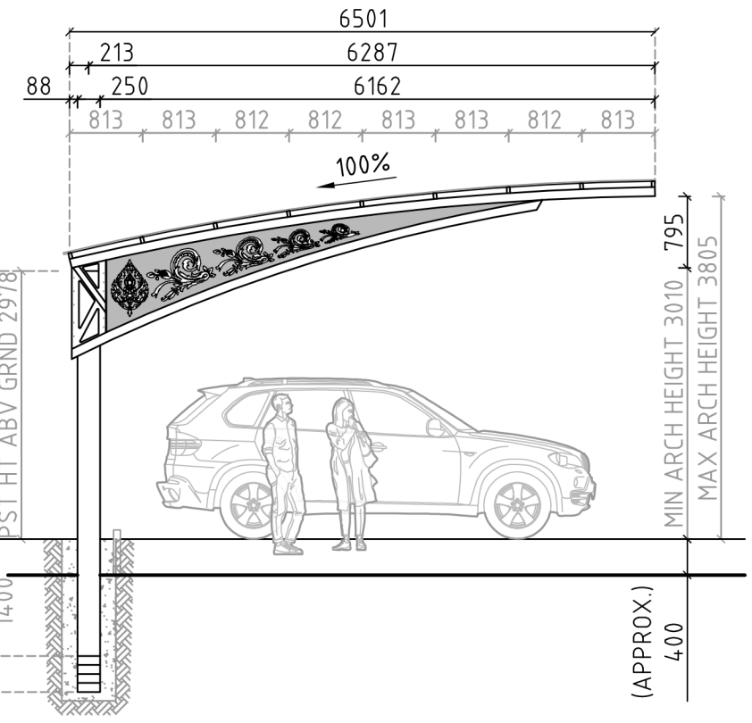
TRUSS ELEVATION
