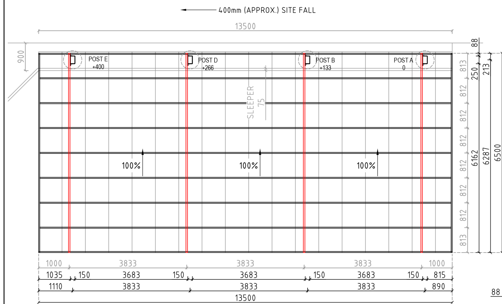
CARPORT PLAN
